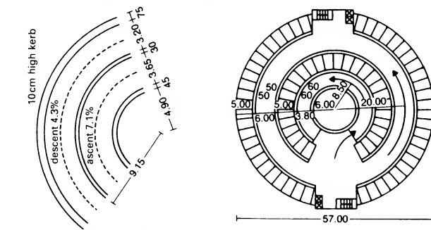
⑤ With smaller radius of ramps, larger lane widths ⑥ Spiral parking ramp
